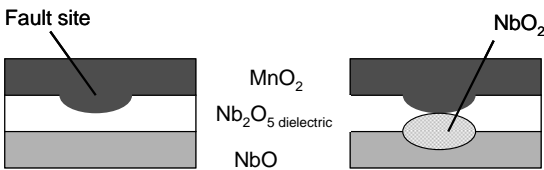
Fig.5. The NbO2 self-arresting process
