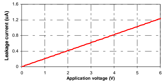
Figure 4: Leakage current representation in V-A characteristic
