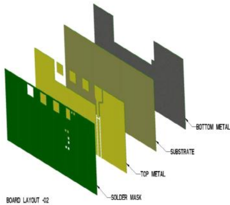
Figure 2 below shows the GNSS PCB Antenna Layout for 1001011_Off-Ground
