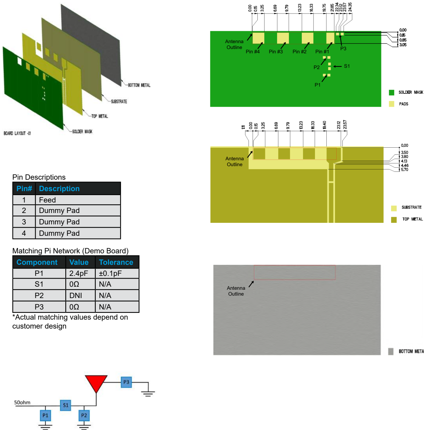
Figure 3: Antenna Layout for 1001011 On-Ground
