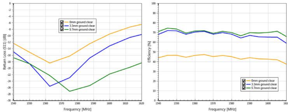
Figure 8: Ground clearance changes for 1001011
