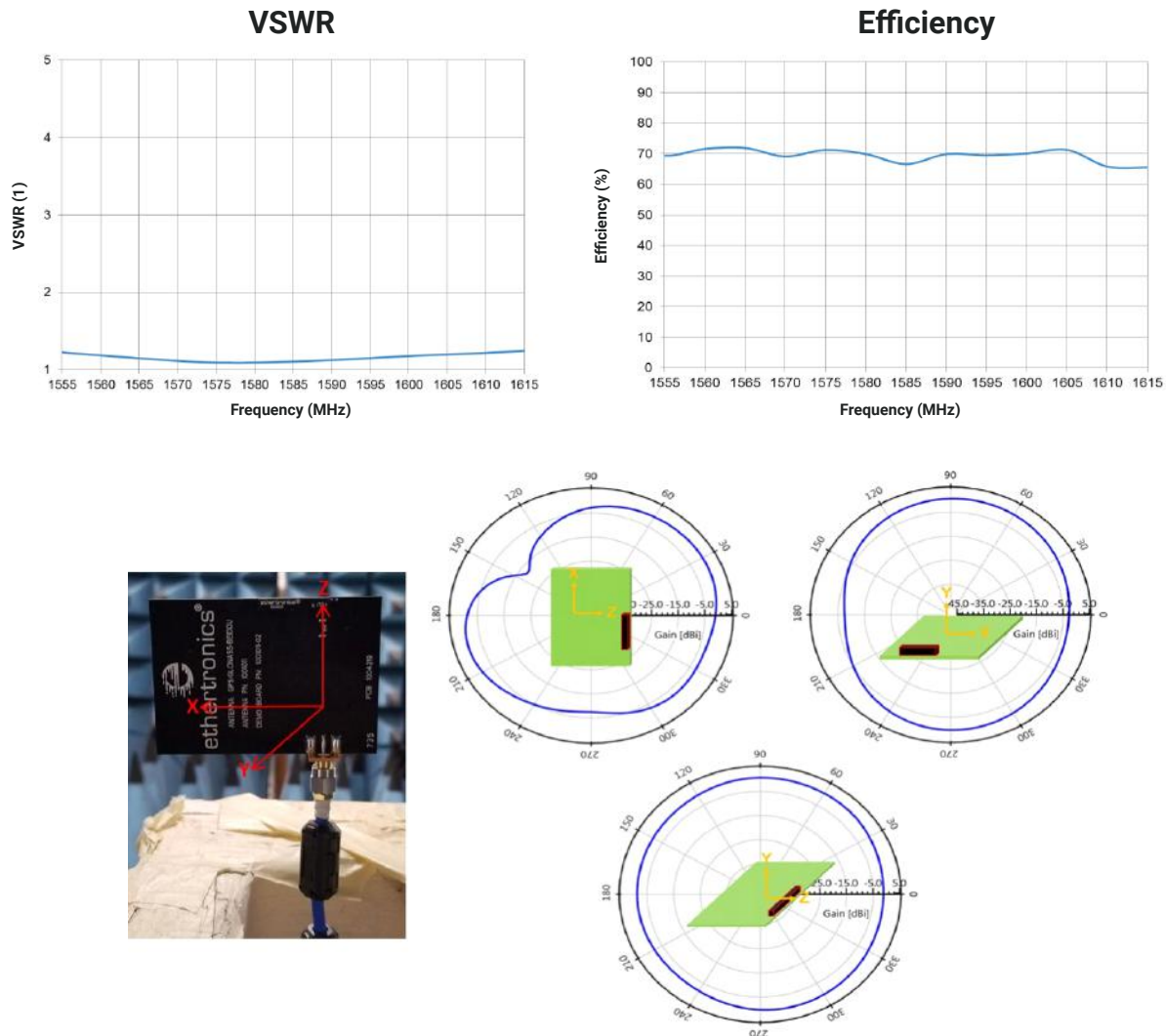
Figure 4: Typical Performance for 1001011_Off-Ground
