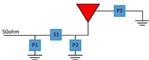
Figure 2: Antenna Layout for 1001011 Off-Ground
