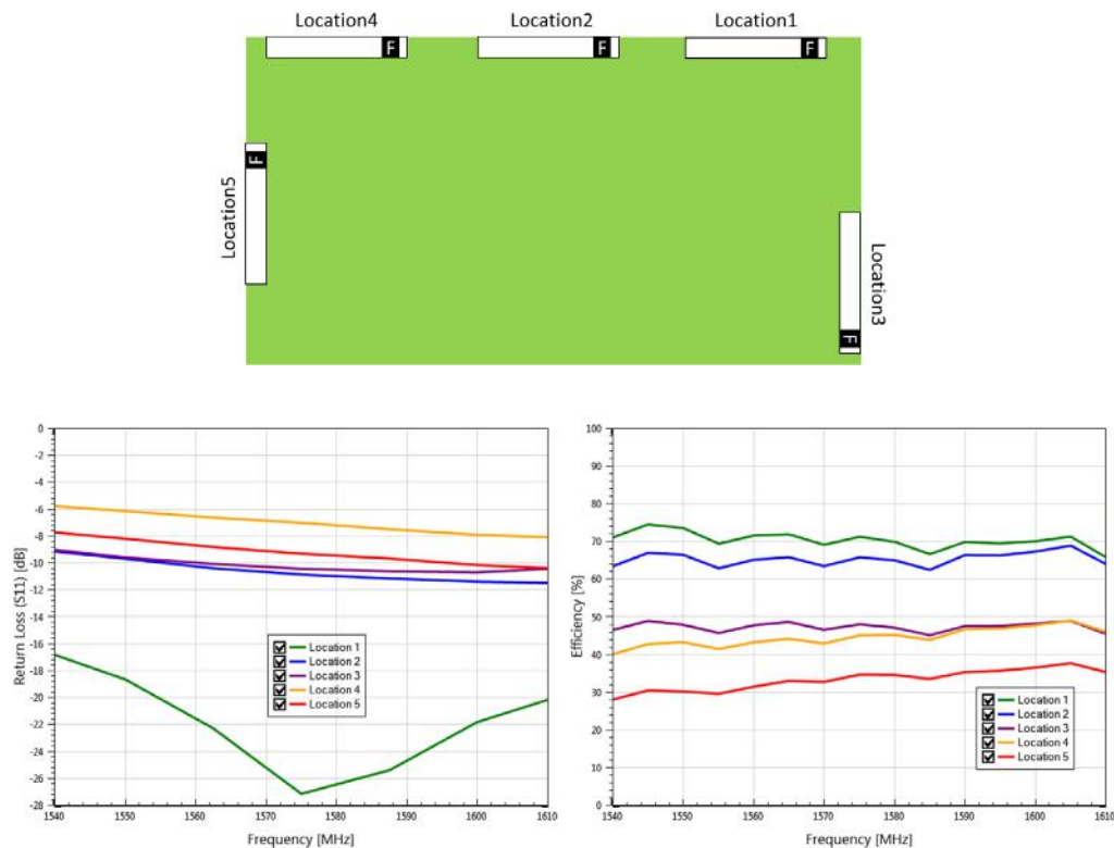
Figure 9: 1001011 antenna on different board locations
