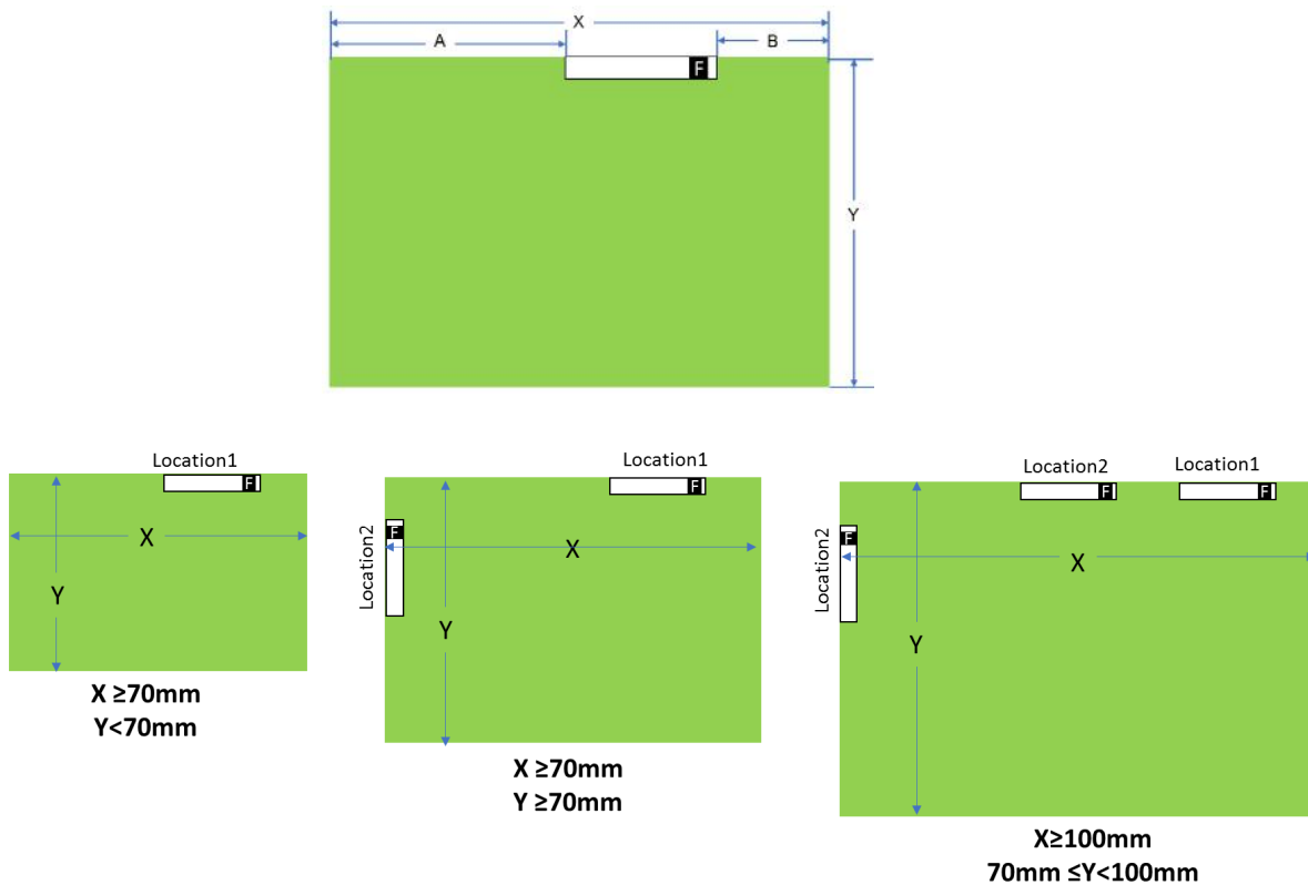
Figure 6: Optimal placement of the 1001011 on a PCB
