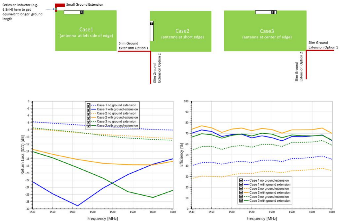
Figure 10: 1001011 antenna performance improvements with ground extensions
