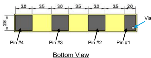
Figure 1 : Antenna Dimensions and Pad Layout for 1001011
