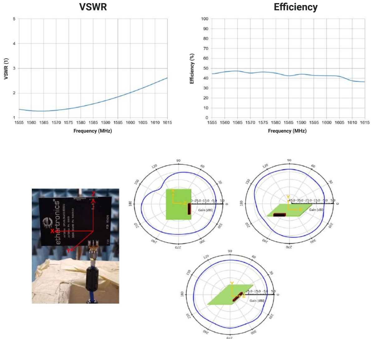
Figure 5: Typical Performance for 1001011_On-Ground
