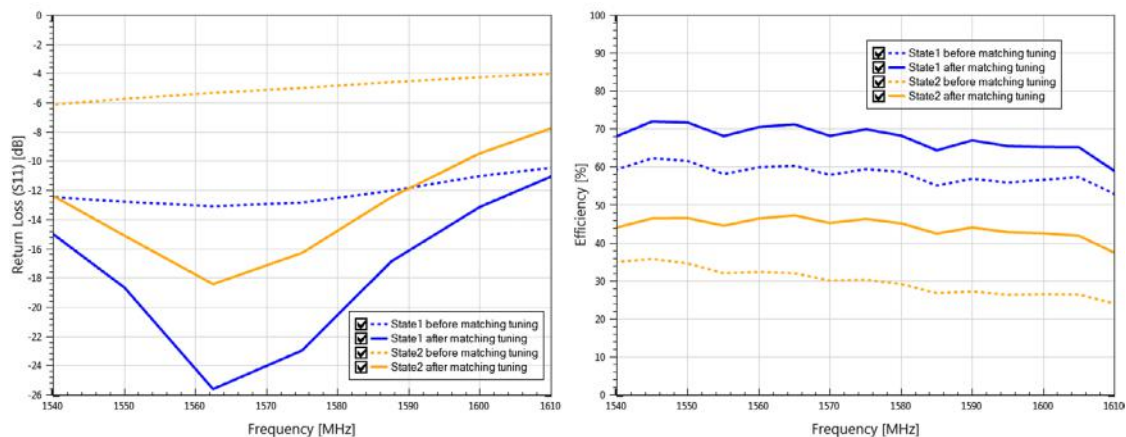
Figure 7: Matching Tuning adjustment for 1001011
