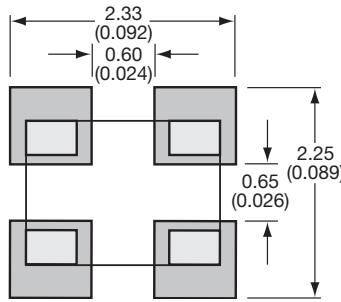
CP0603 LGA
