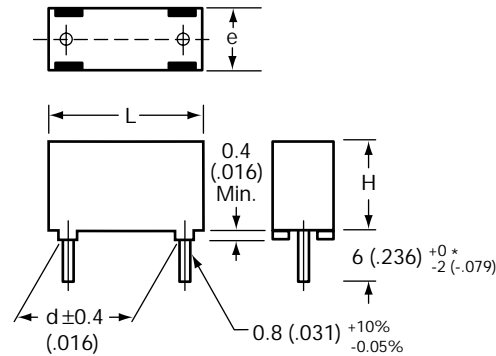
Dimensions mm (inches) *Other lead lengths upon request
